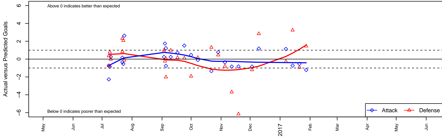
Crossfire Select Zlatko B03 Dots are actual minus expected GF (blue circles) and GA (red triangles). Blue line is smoothed change in attack strength. Red is smoothed change in defense strength.
